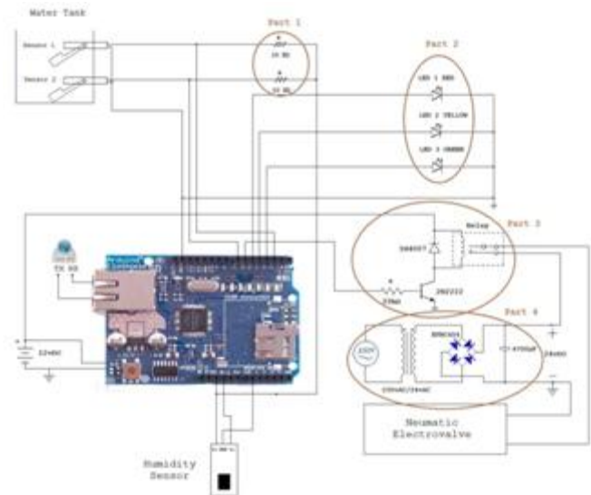
Figure 13: Electric circuits
