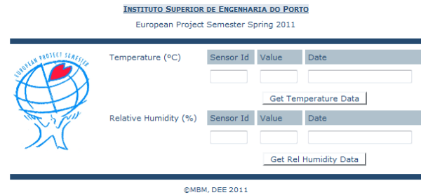
Figure 16: Web interface
