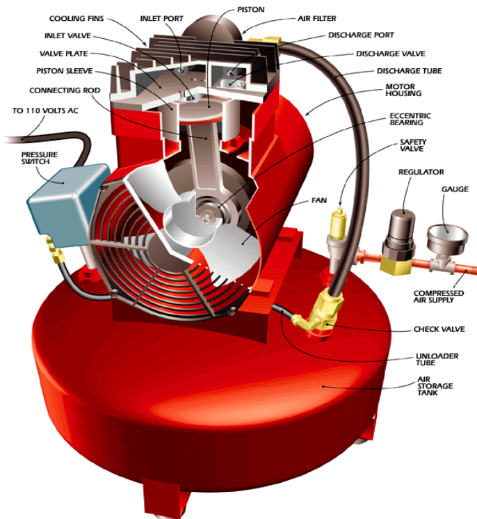
Figure 3: Parts of a compressor
